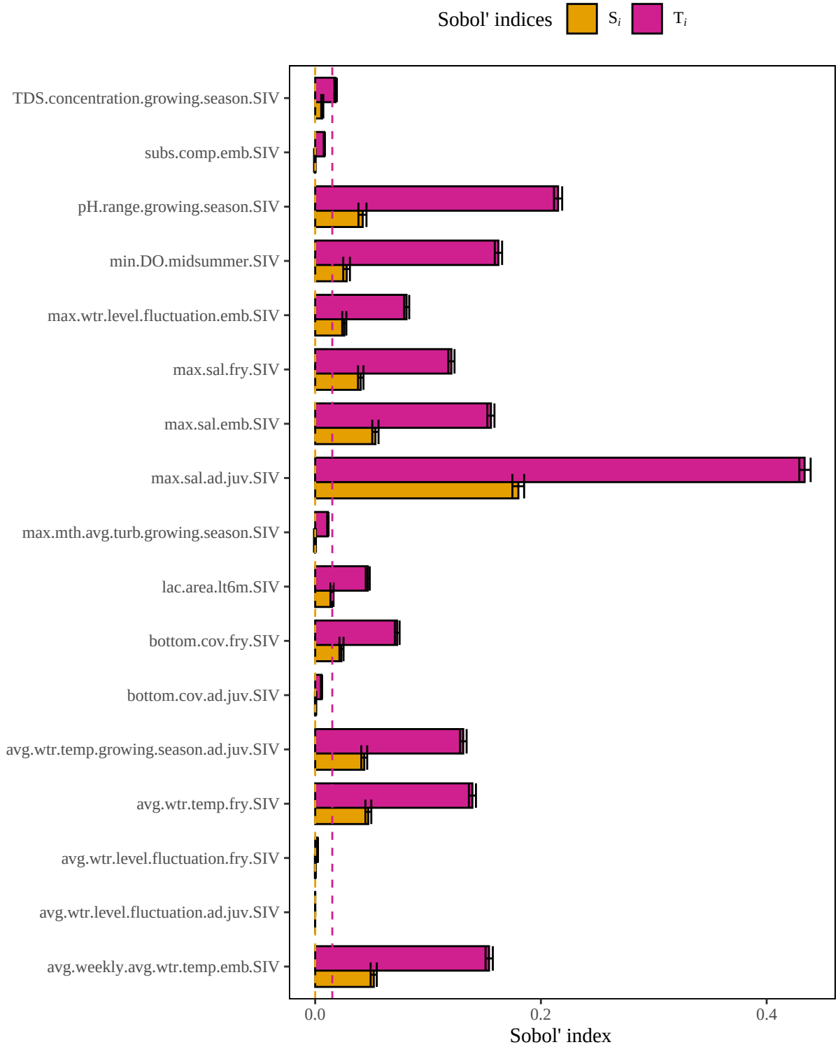
Figure 6. Results of a sensitivity analysis for the largemouthbassLacN model based on a limiting factor structure. Dashed lines represent baseline numerical approximation error for S_i and T_i ( i.e. , dummy variables).
