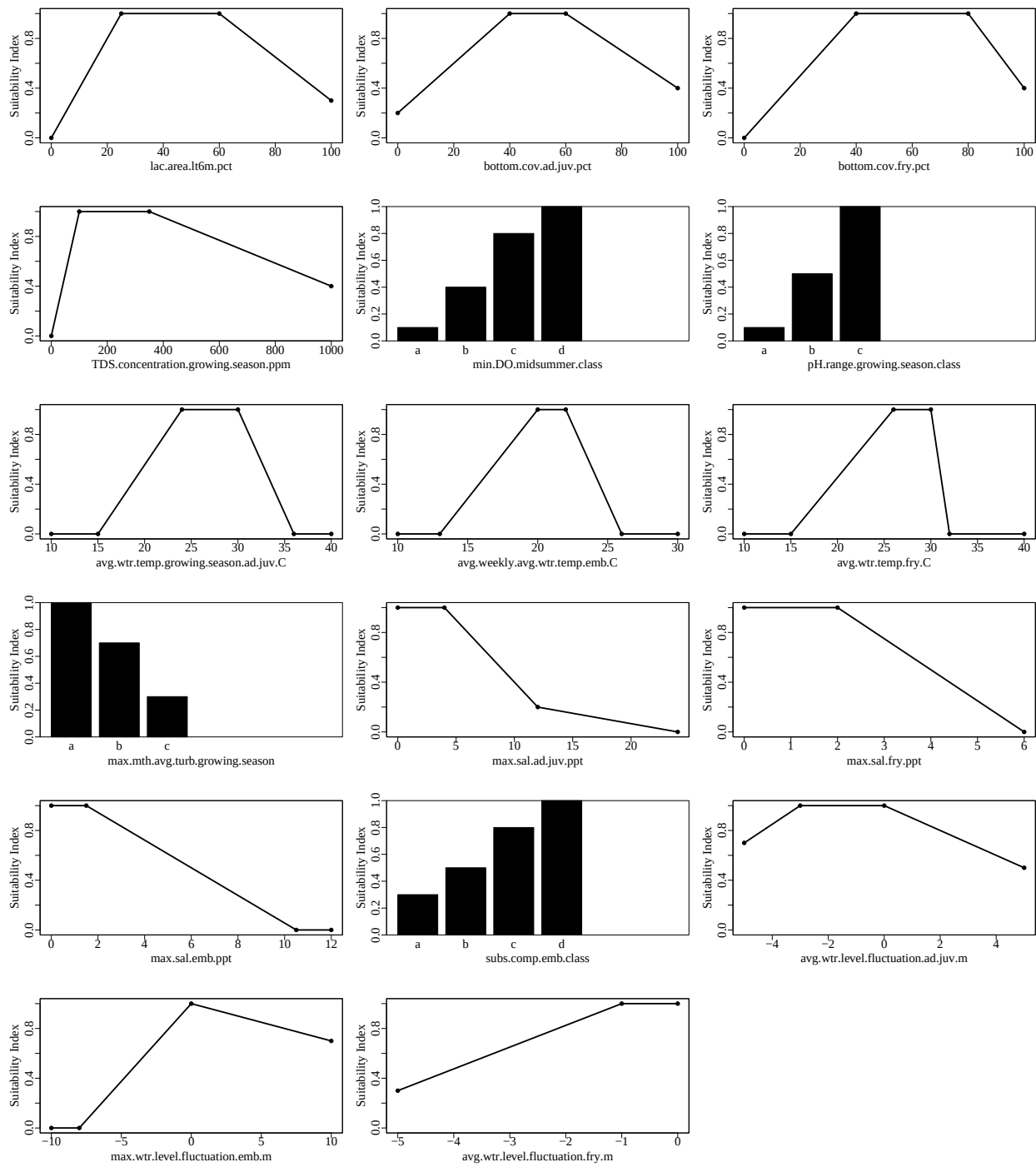
Figure 1. Suitability index graphs for variables included in the largemouthbassLacN model in ecorest.
