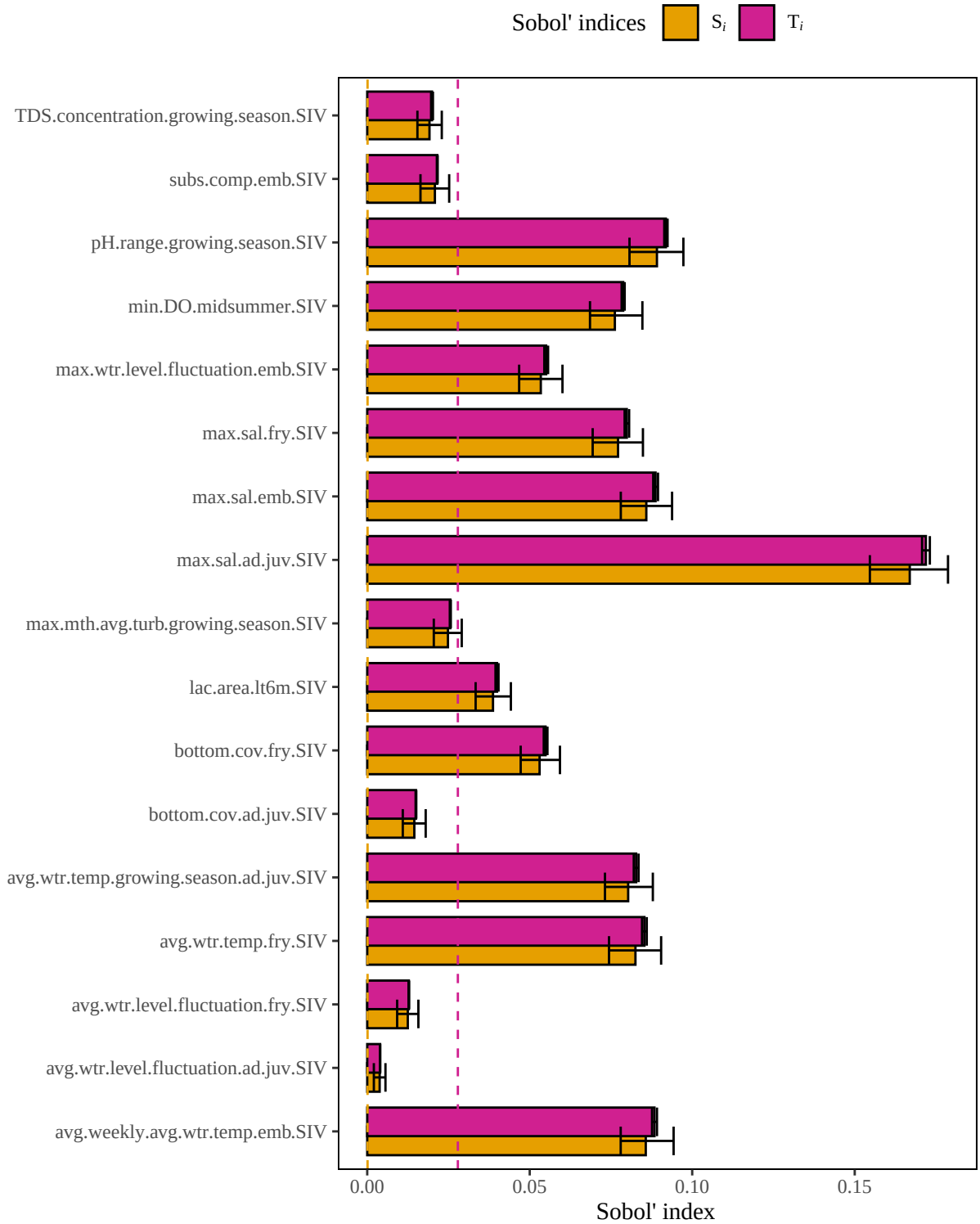
Figure 5. Results of a sensitivity analysis for the largemouthbassLacN model based on a geometric mean structure. Dashed lines represent baseline numerical approximation error for S_i and T_i ( i.e. , dummy variables).
